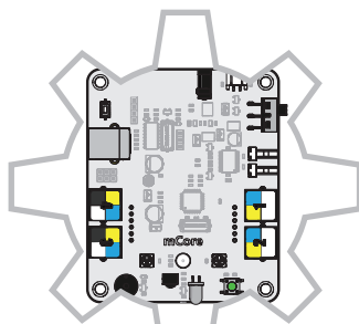
mCore Layout
