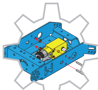
Assembly Instructions
